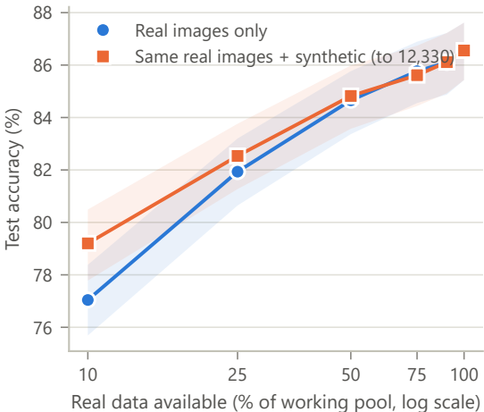
a Accuracy vs. amount of real data
