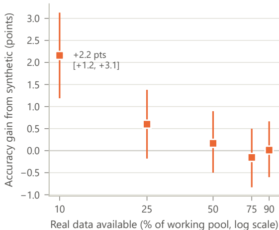
b What the synthetic images add (paired, 95% CI)
