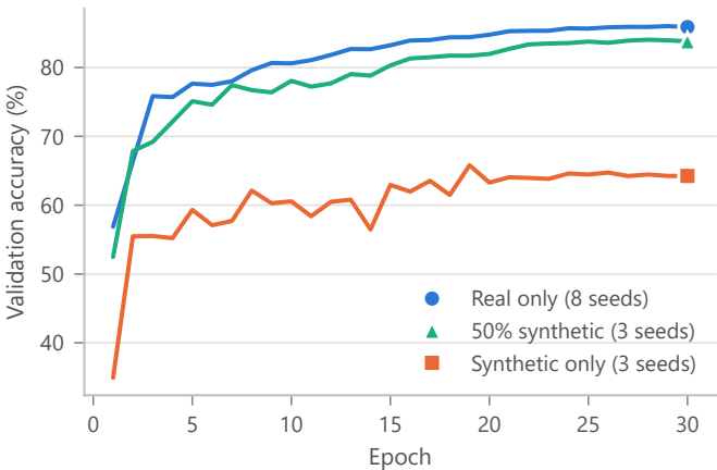
Classifier training curves (seed mean)
