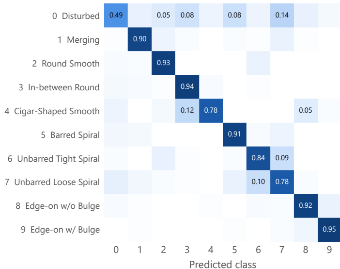
Trained on real only (8 seeds pooled)
