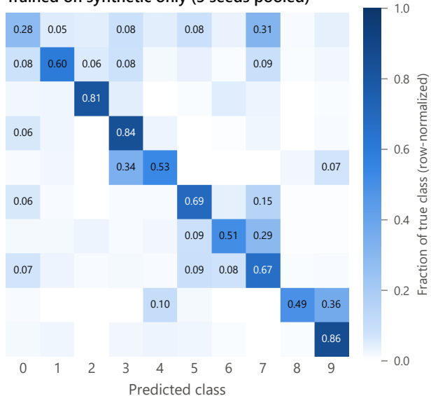
Trained on synthetic only (3 seeds pooled)
