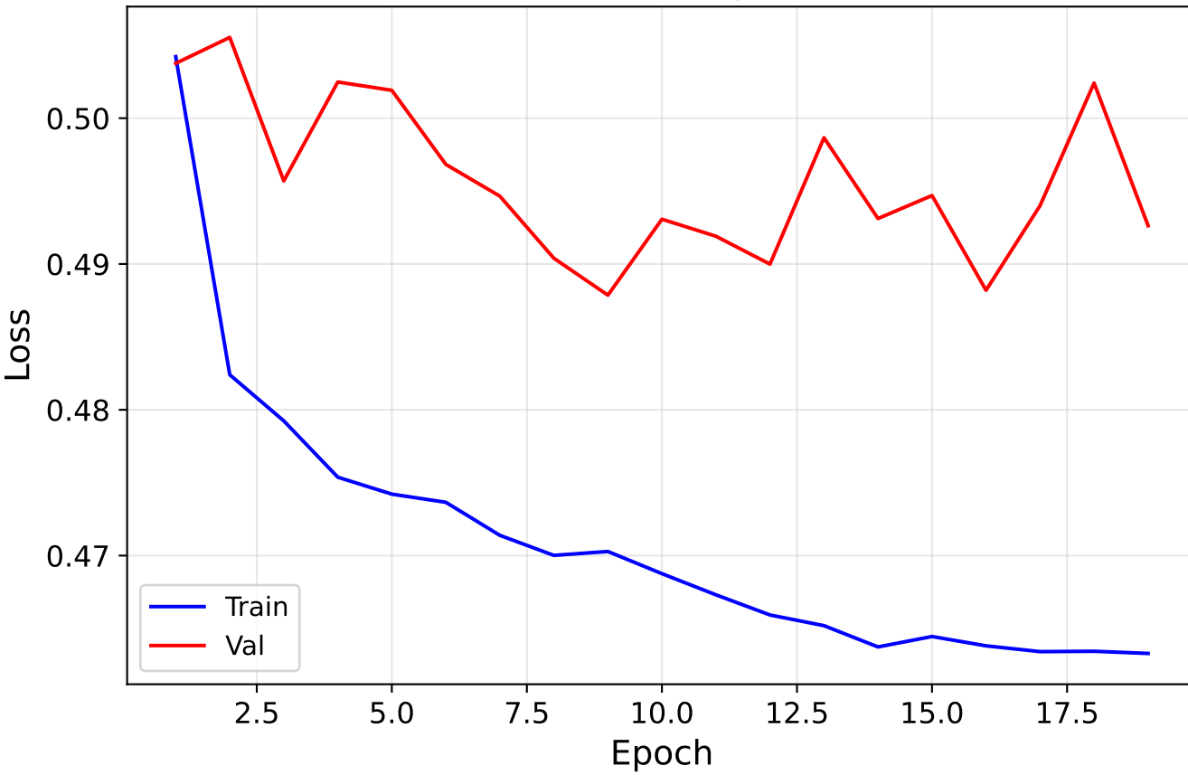
DEAP Pretraining — Loss
