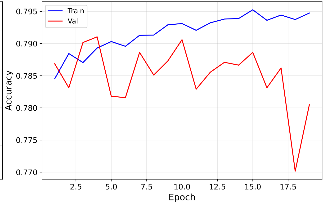
DEAP Pretraining — Accuracy
