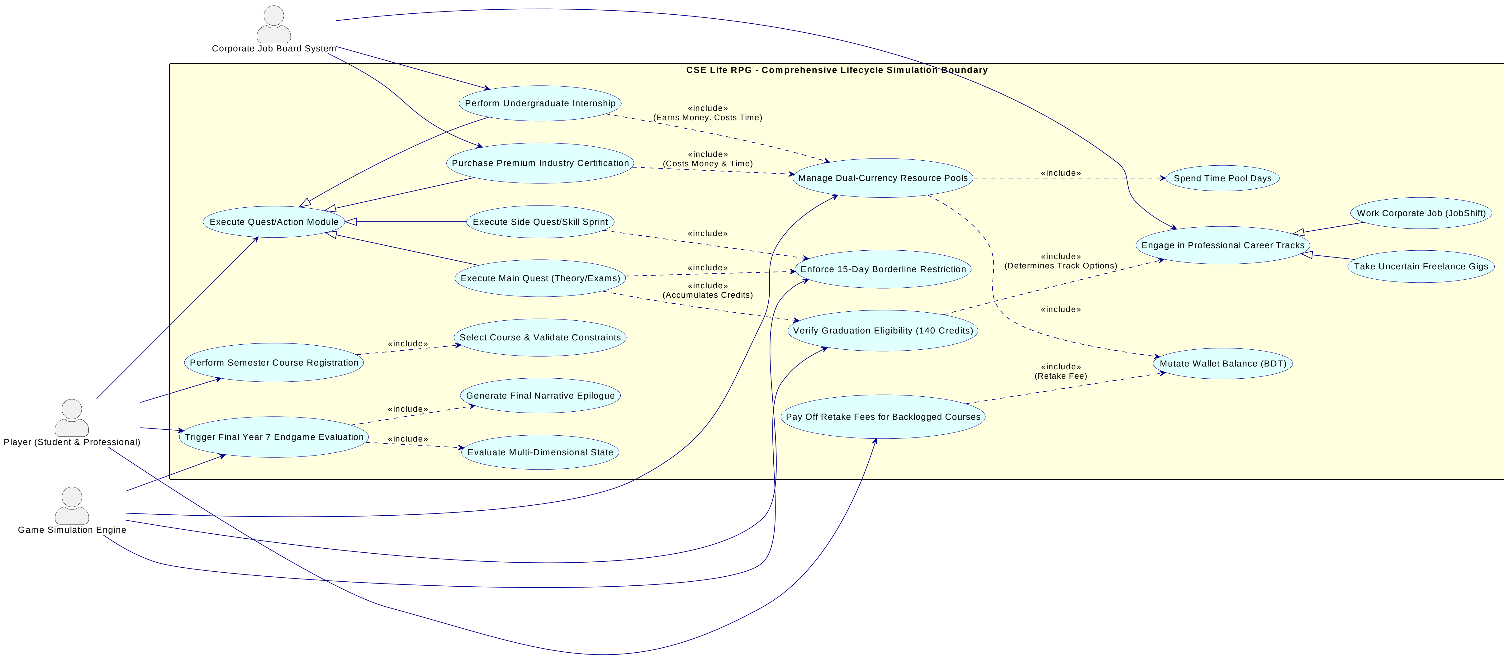
CSE Life RPG - Extended Ultimate Game Use Case Diagram (Phase 1 & Phase 2)
