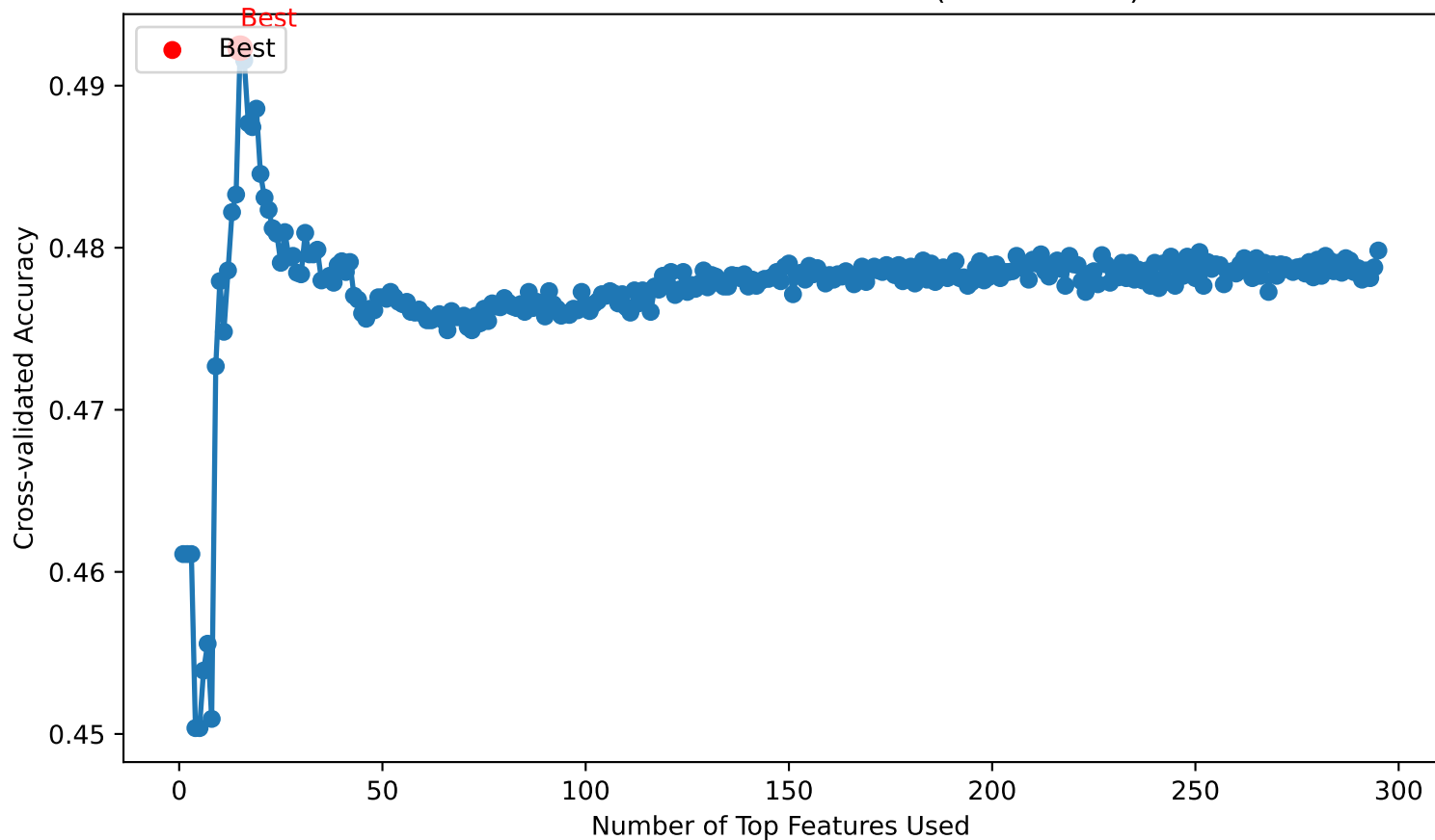
Decision Tree Attribute Selection (Full Dataset)
