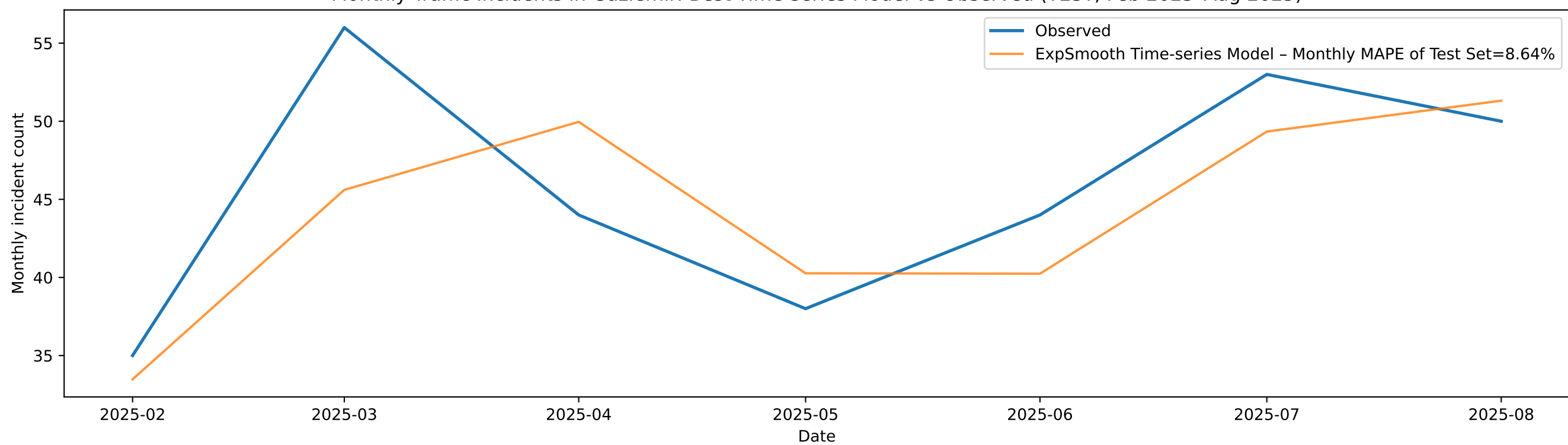
Monthly Traffic Incidents in Gaziemir: Best Time-series Model vs Observed (TEST, Feb 2025-Aug 2025)
