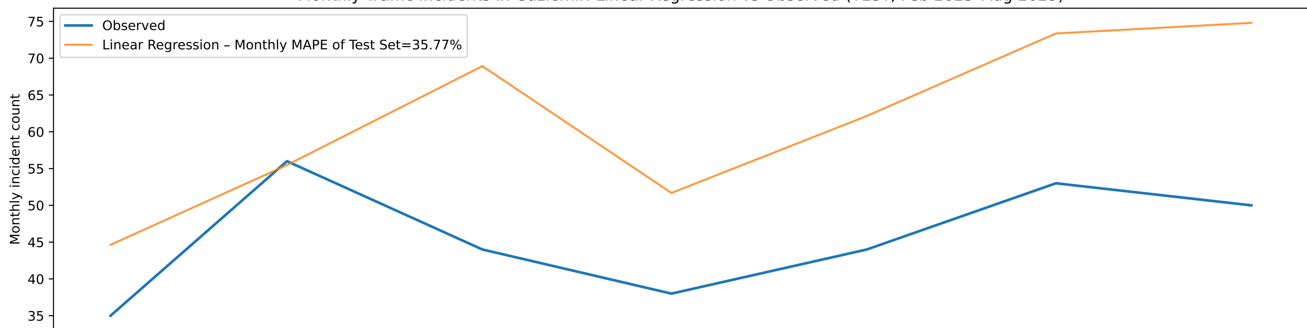
Monthly Traffic Incidents in Gaziemir: Best Time-series Model vs Observed (TEST, Feb 2025-Aug 2025)
