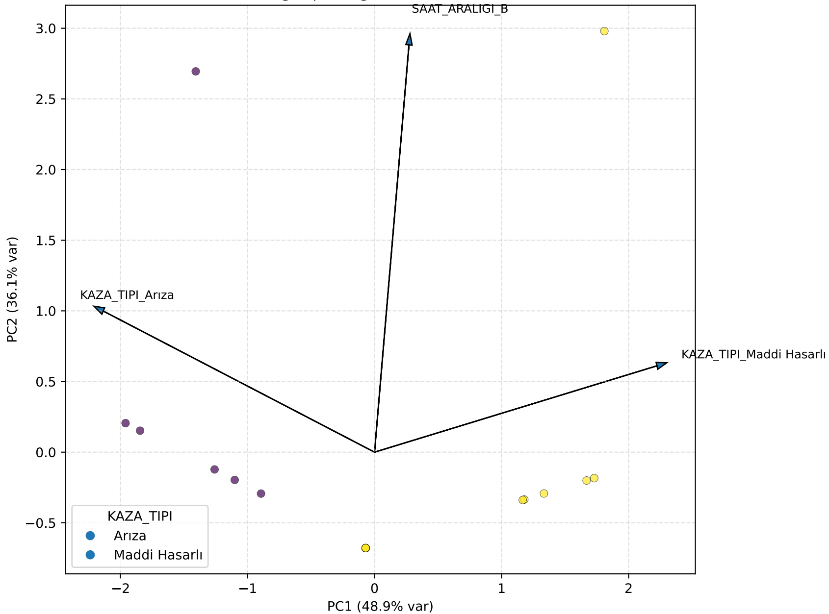
PCA using Top-3 Highest-Variance Features
