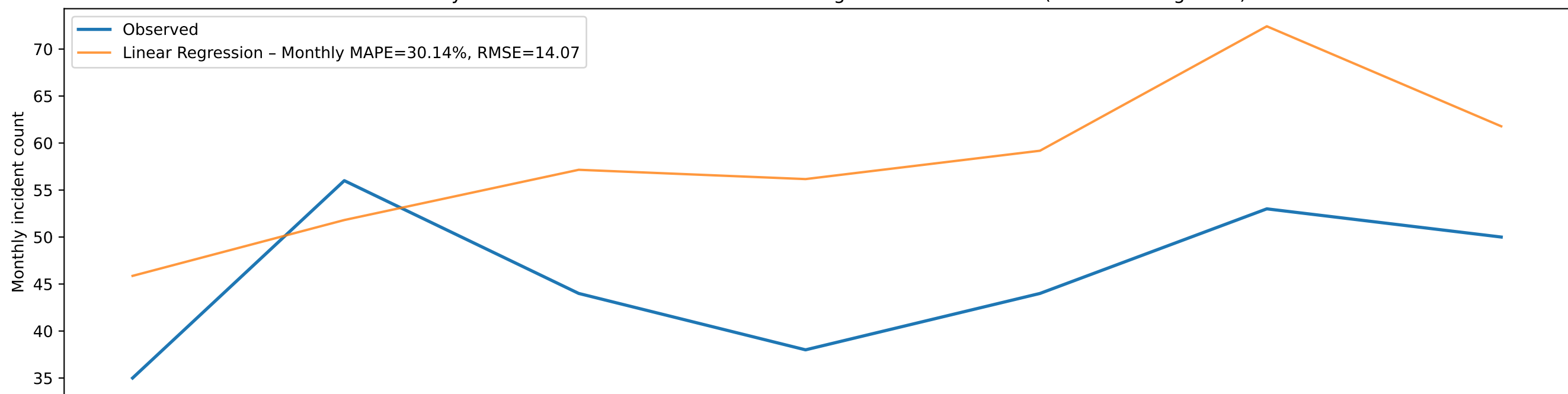
Monthly Traffic Incidents in Gaziemir: Best Time-series Model vs Observed (Feb 2025-Aug 2025)
