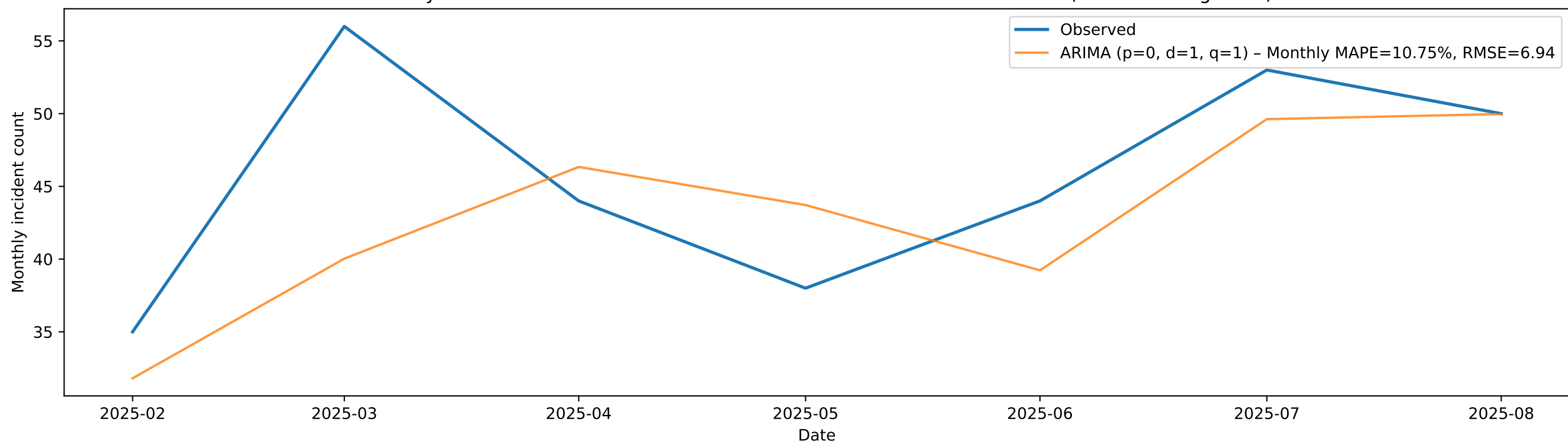
Monthly Traffic Incidents in Gaziemir: Best Time-series Model vs Observed (Feb 2025-Aug 2025)
