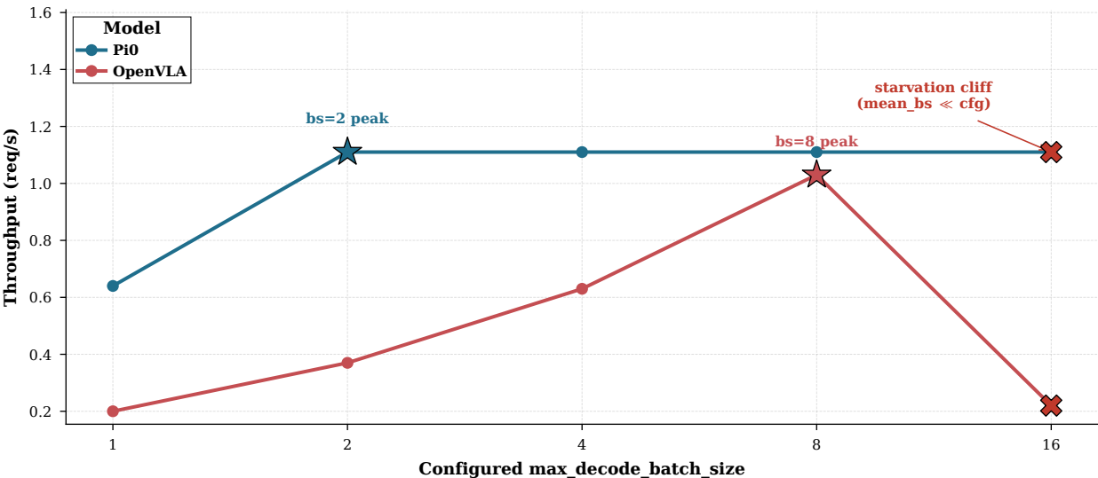
E6 — Throughput vs configured batch size
