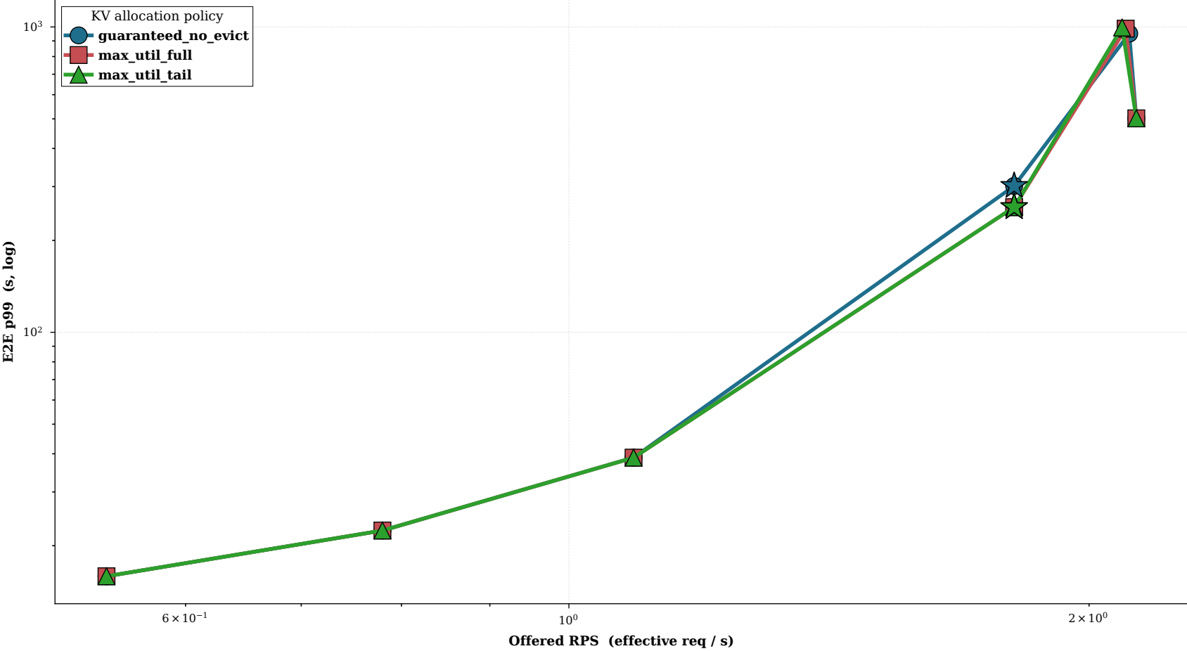
Pi0 @ azure_poisson_wide v2 — knee vs KV allocation policy
