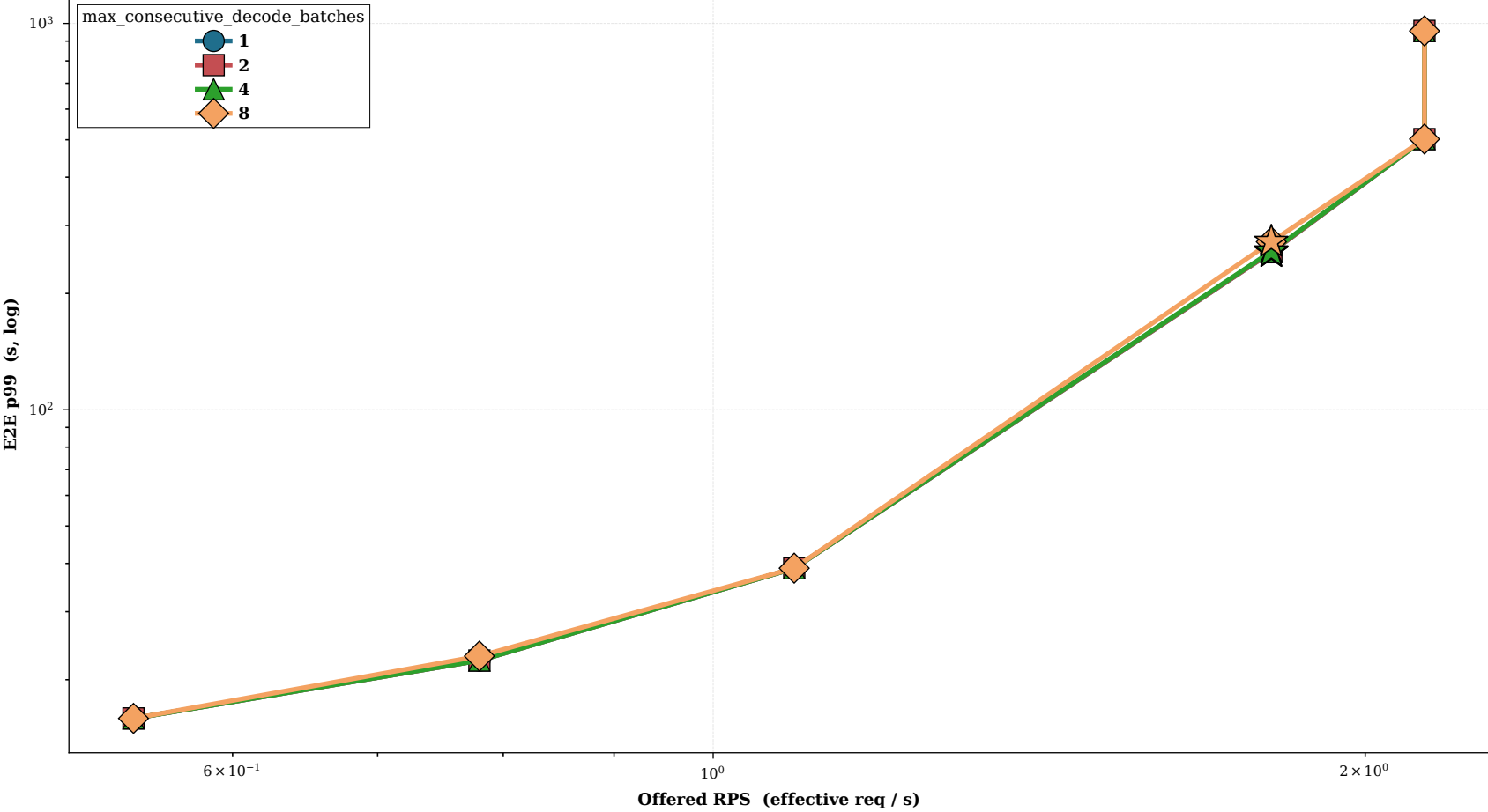
Pi0 @ azure_poisson_wide v2 — knee vs max_consecutive_decode_batches
