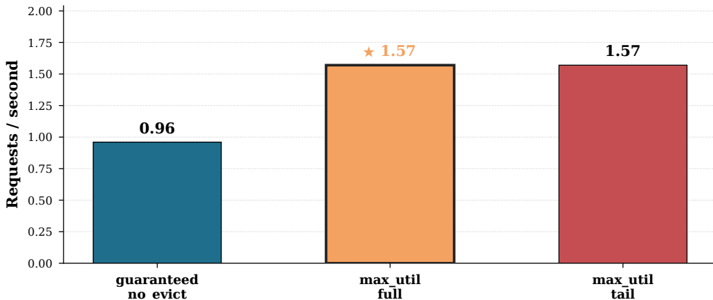
(c) Admitted requests (aggression)
