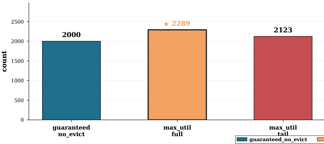
(c) Admitted requests (aggression)
