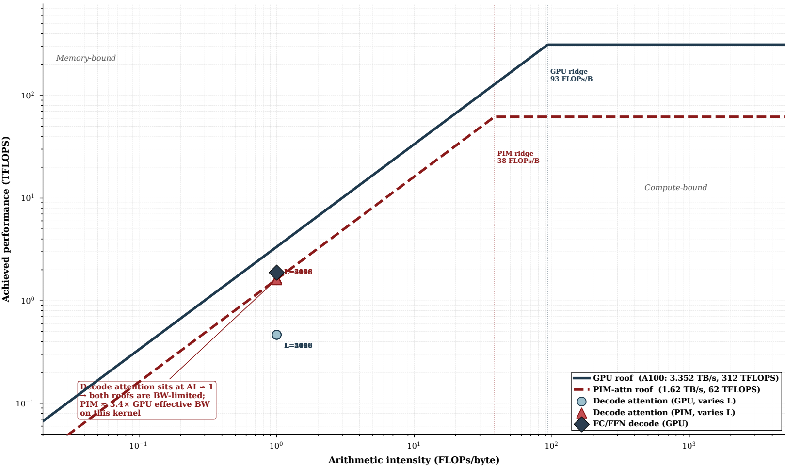
Roofline — Pi0 attention on A100 GPU vs LPDDR5-PIM (bs=1)
