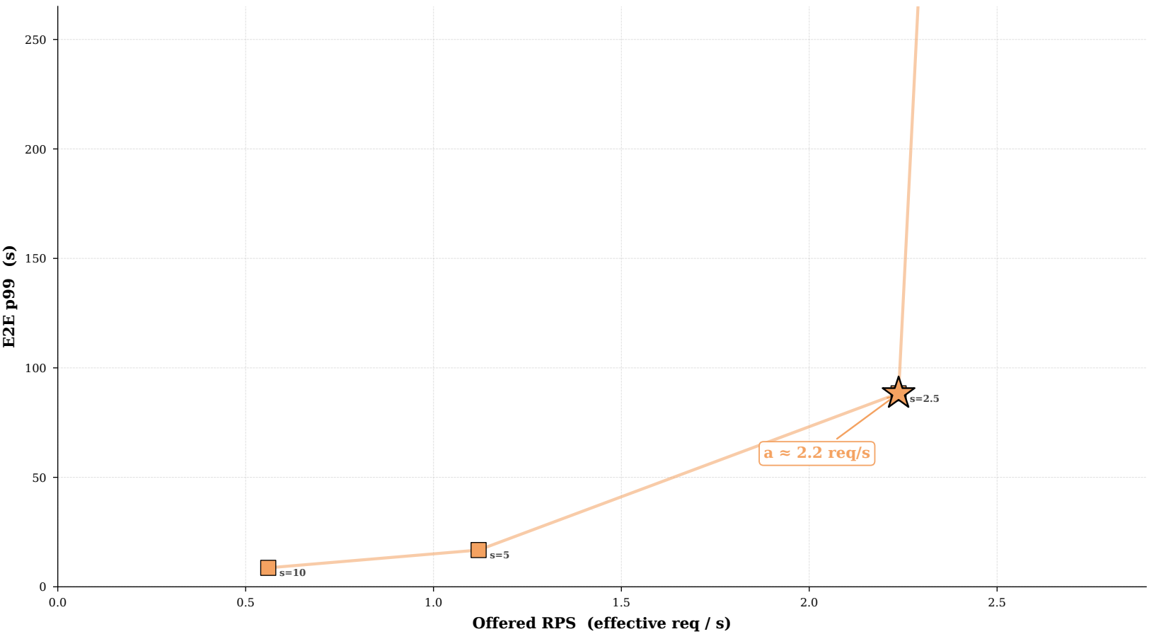
Azure (Poisson shape) — peak-RPS knee (linear axes — y capped at 3\times knee p99)
