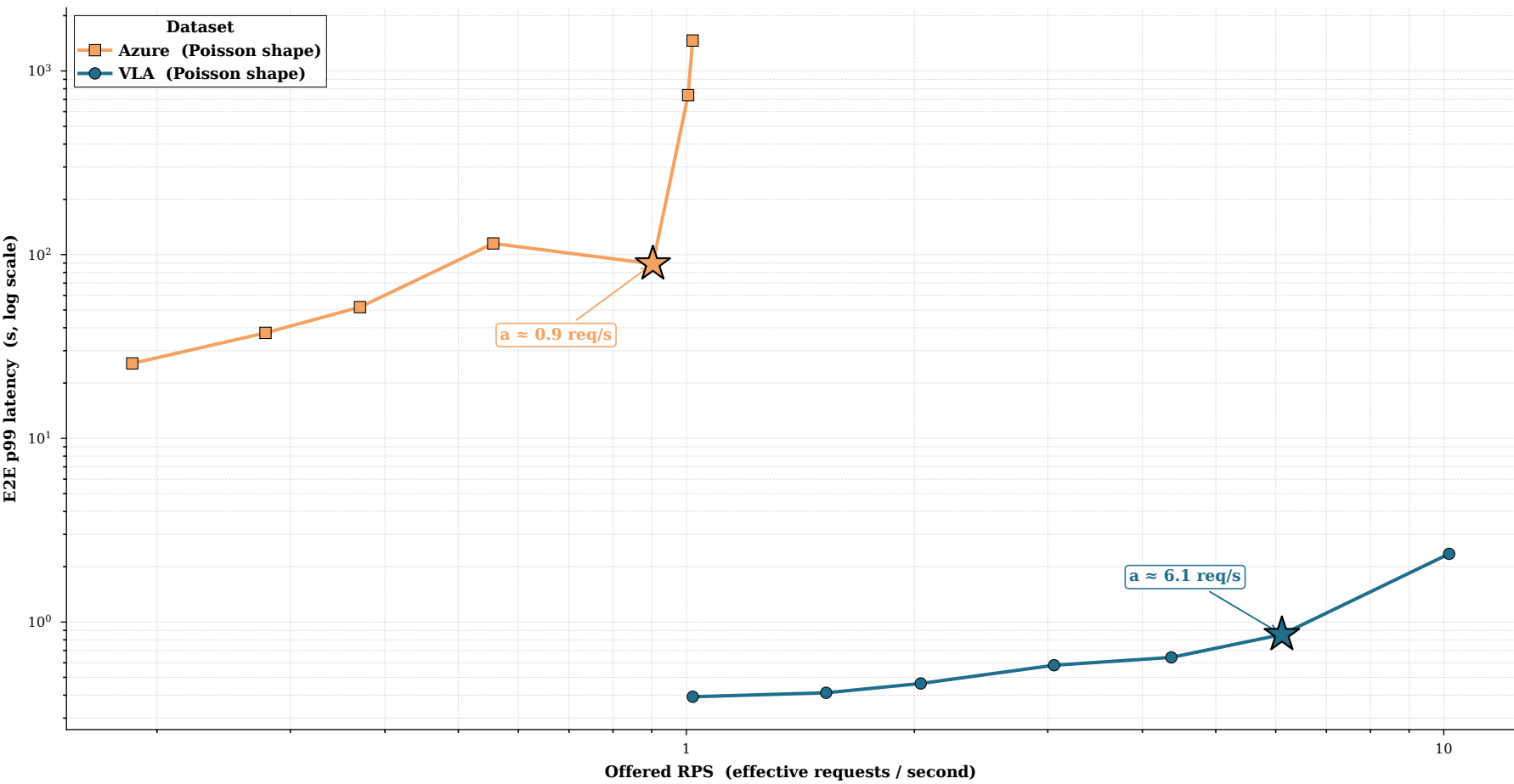
Peak-RPS knee — where the system saturates
