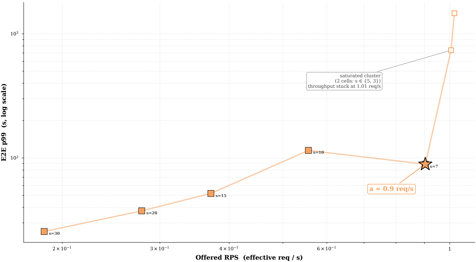
Azure (Poisson shape) — peak-RPS knee (s = arrival_scale; a = knee/sustainable peak RPS)
