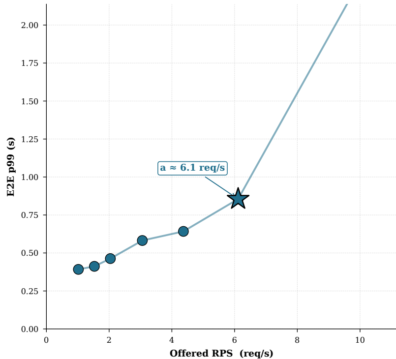
Peak-RPS knee (linear axes — y capped at 2.5 \times knee p99) Azure (Poisson shape) VLA (Poisson shape)
