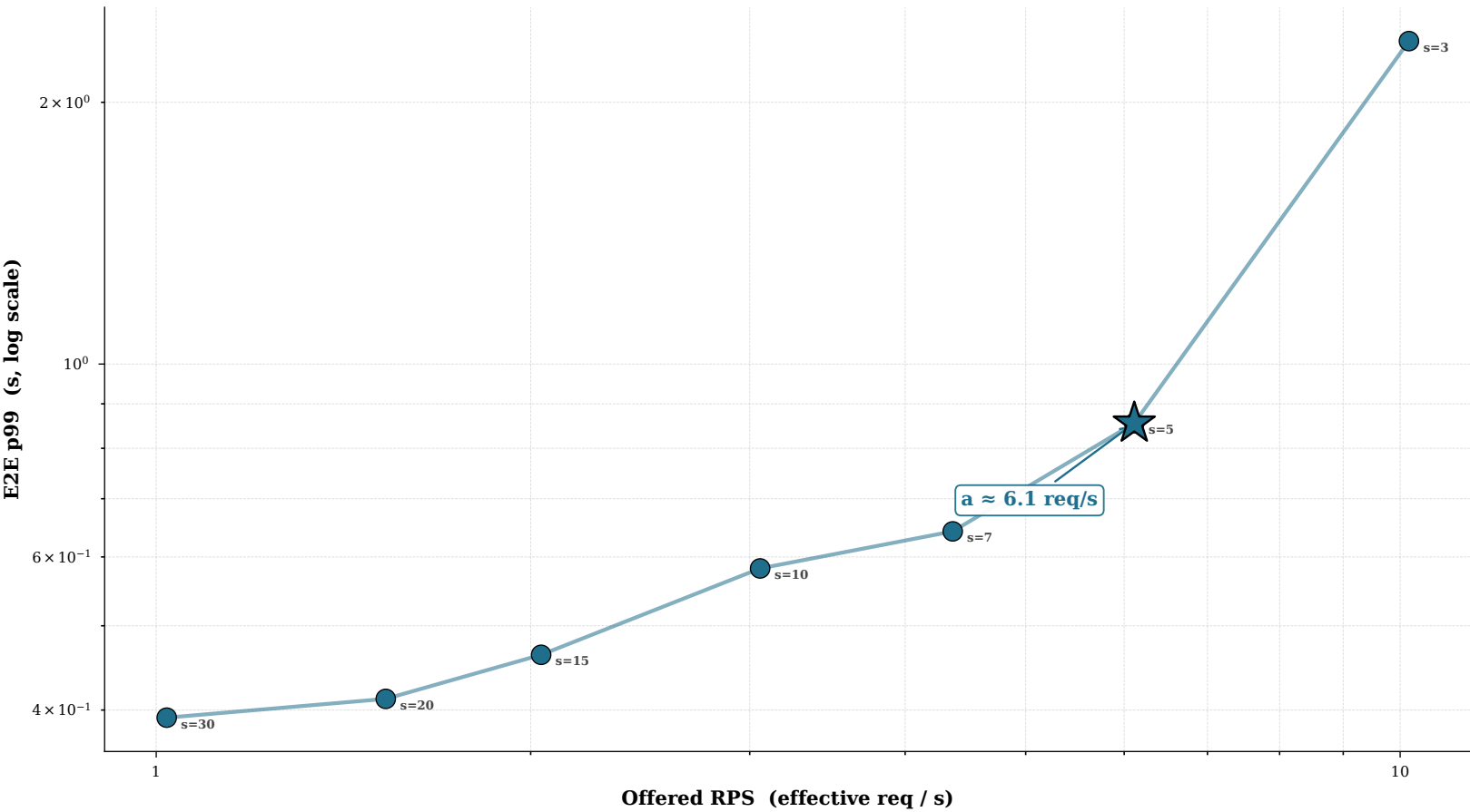
VLA (Poisson shape) — peak-RPS knee (s = arrival_scale; a = knee/sustainable peak RPS)
