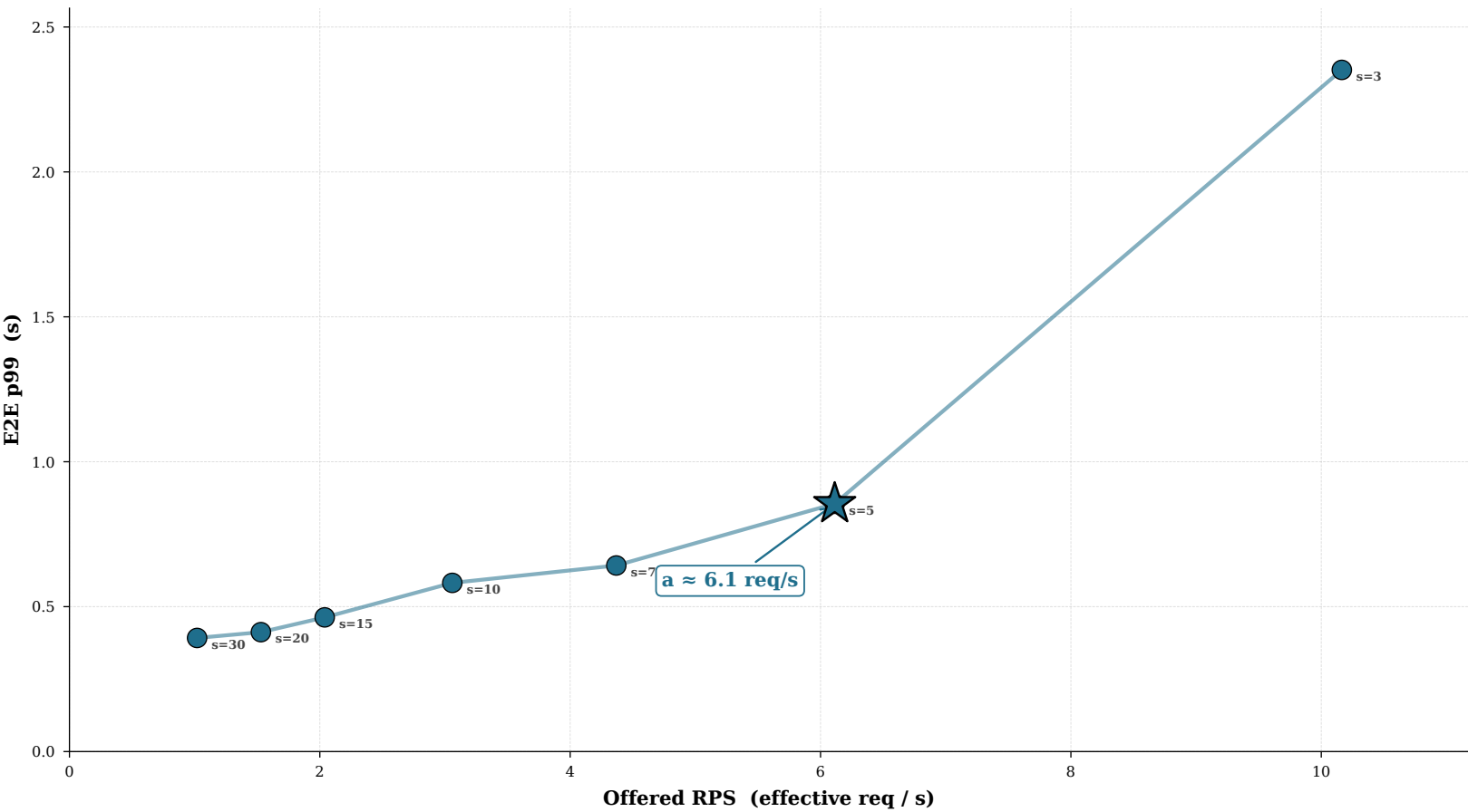
VLA (Poisson shape) — peak-RPS knee (linear axes — y capped at 3\times knee p99)
