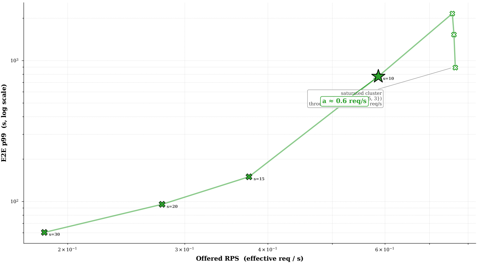
Azure (Poisson, wide mixture) — peak-RPS knee (s = arrival_scale; a = knee/sustainable peak RPS)
