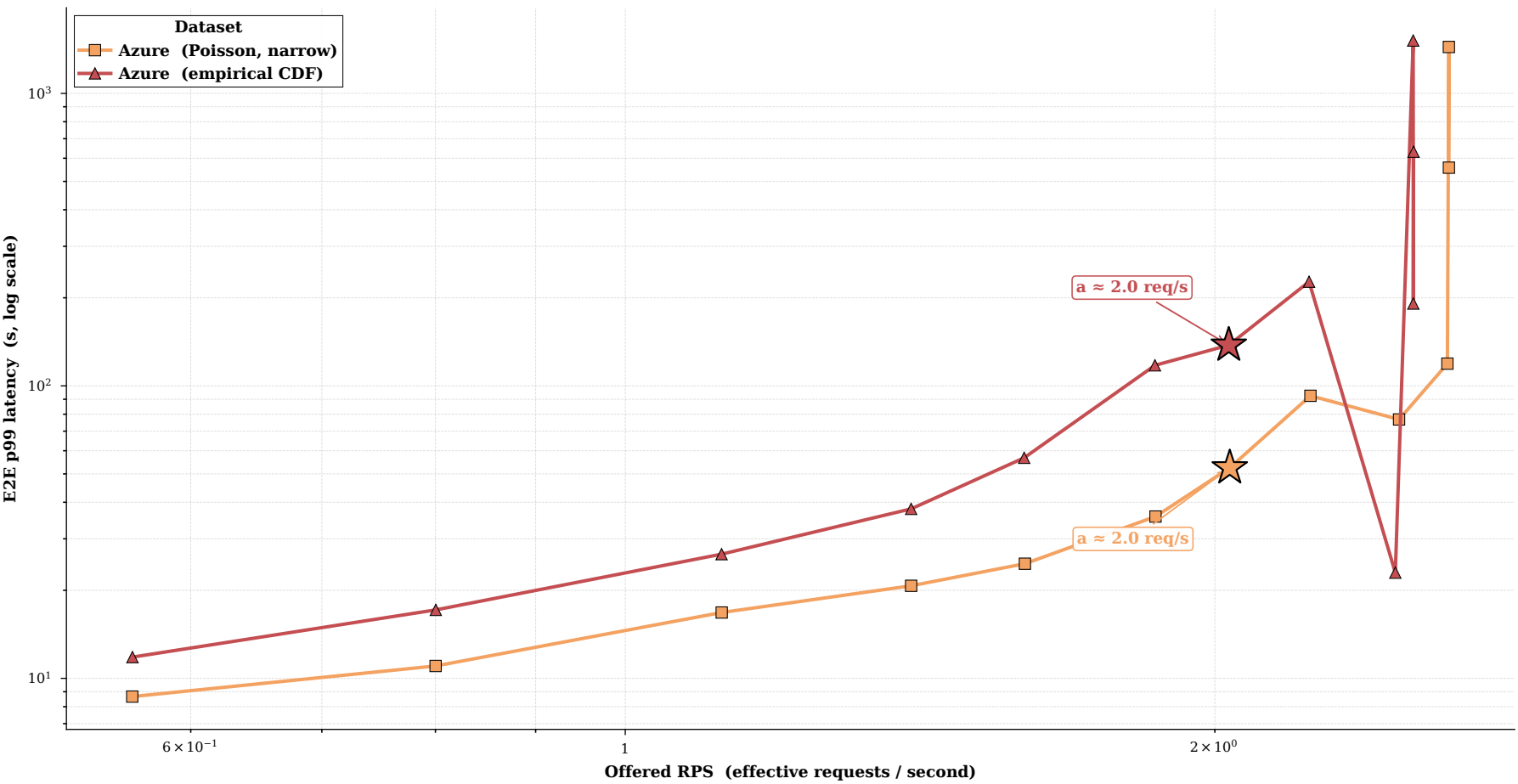
Peak-RPS knee — where the system saturates
