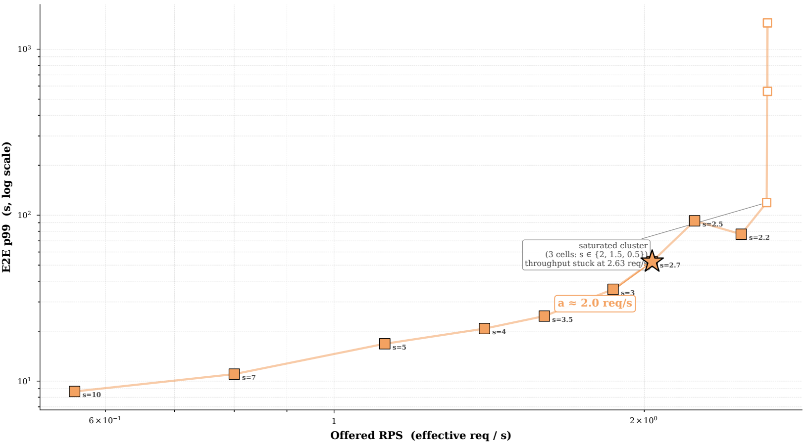
Azure (Poisson, narrow) — peak-RPS knee (s = arrival_scale; a = knee/sustainable peak RPS)
