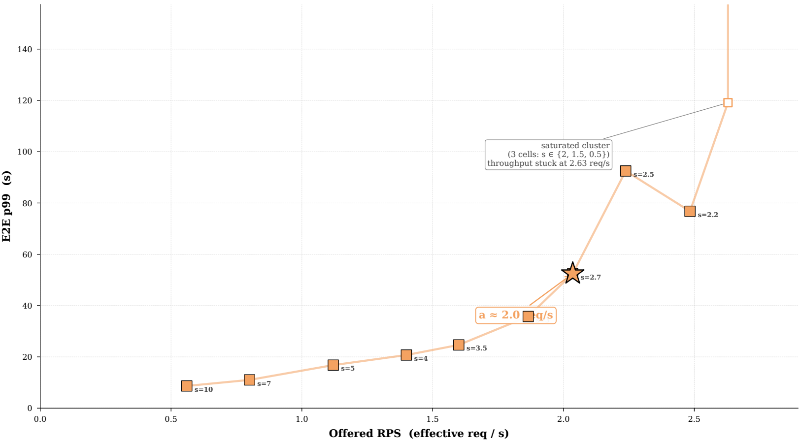
Azure (Poisson, narrow) — peak-RPS knee (linear axes — y capped at 3\times knee p99)
