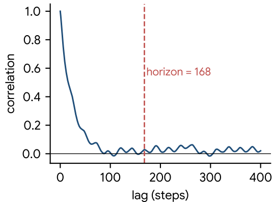
Autocorrelation of the target
