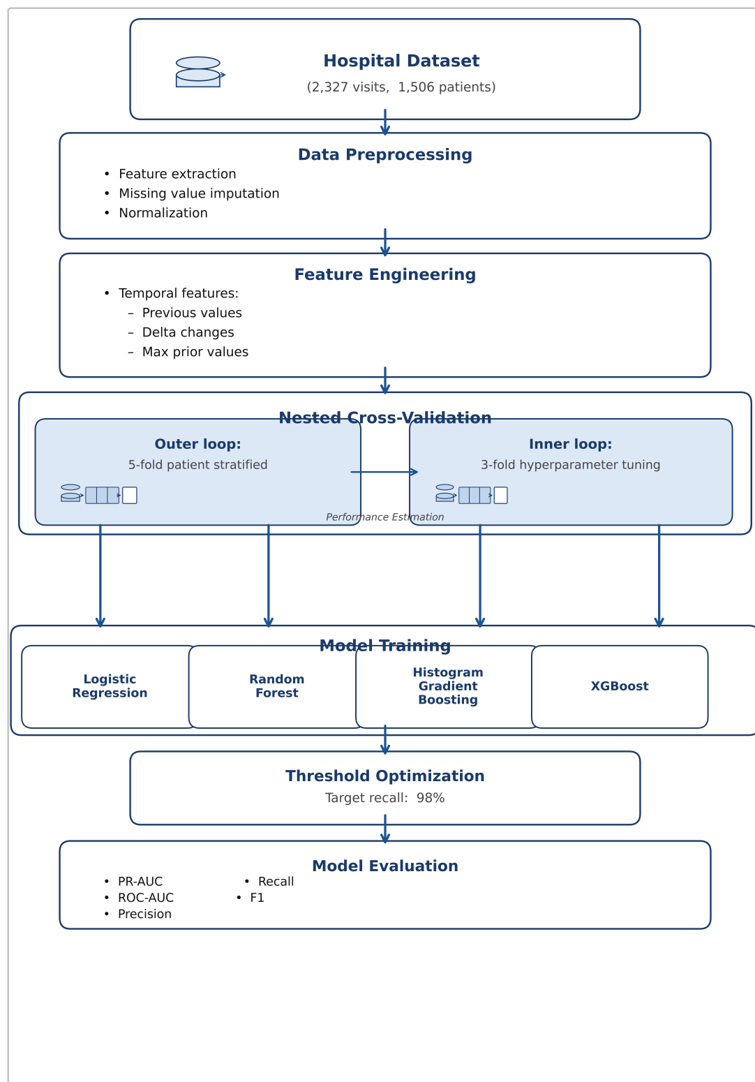
Figure 1. Workflow diagram of the proposed MI detection methodology. The pipeline includes data preprocessing, temporal feature engineering, nested cross-validation with patient-level stratification, training of four ML classifiers, threshold optimization for 98% recall, and comprehensive model evaluation.
