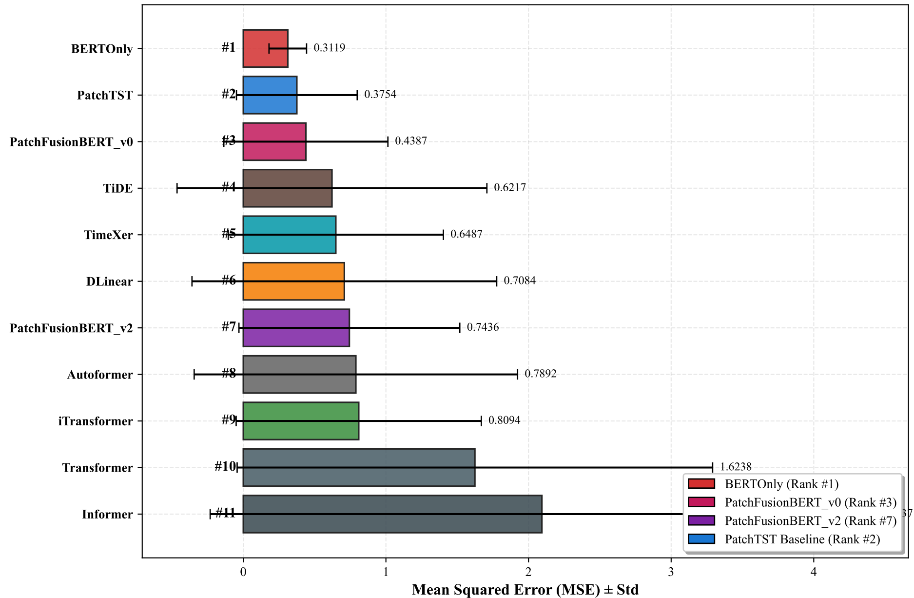
Overall Model Performance Ranking Across All Datasets
