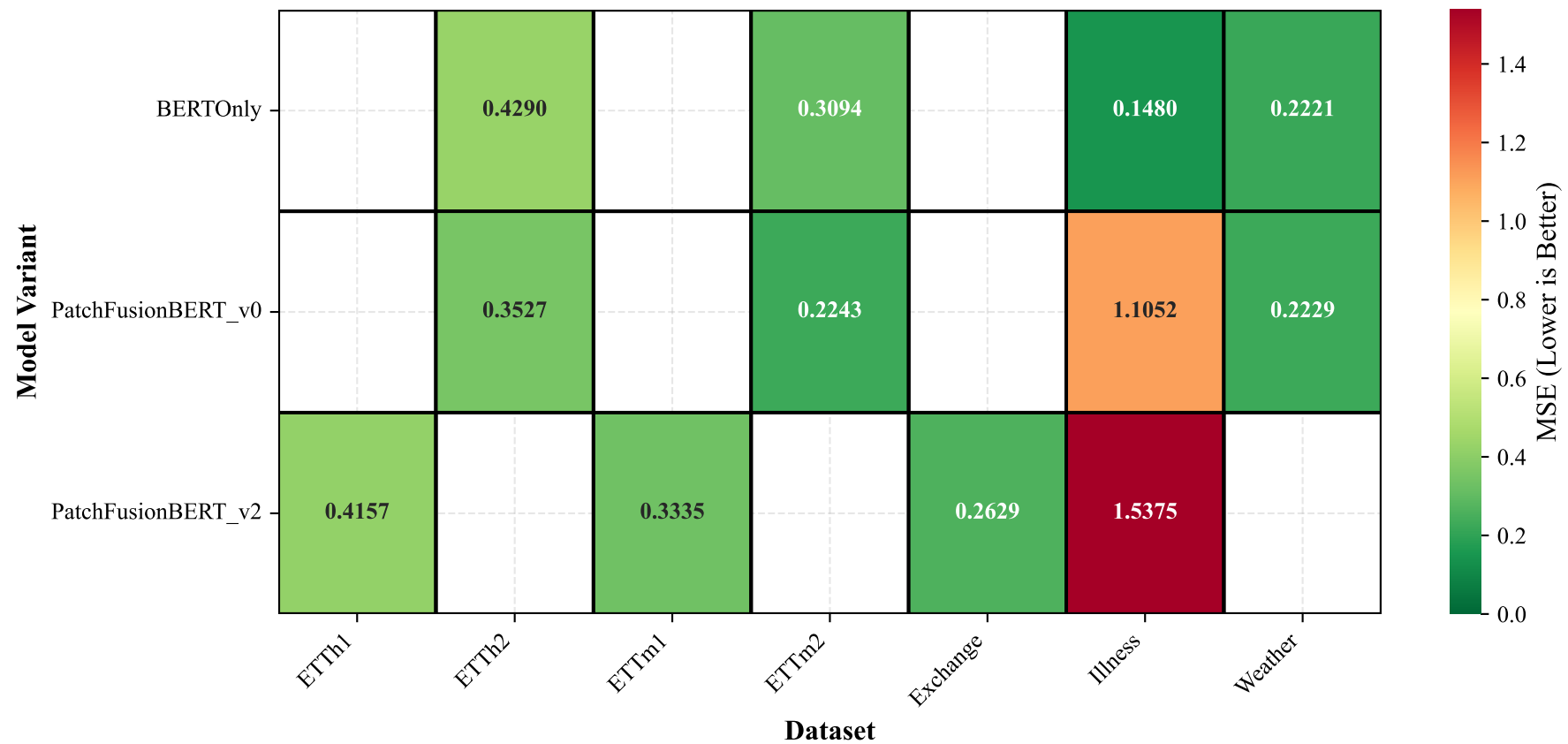
PatchFusionBERT Variants: Dataset-Wise Performance
