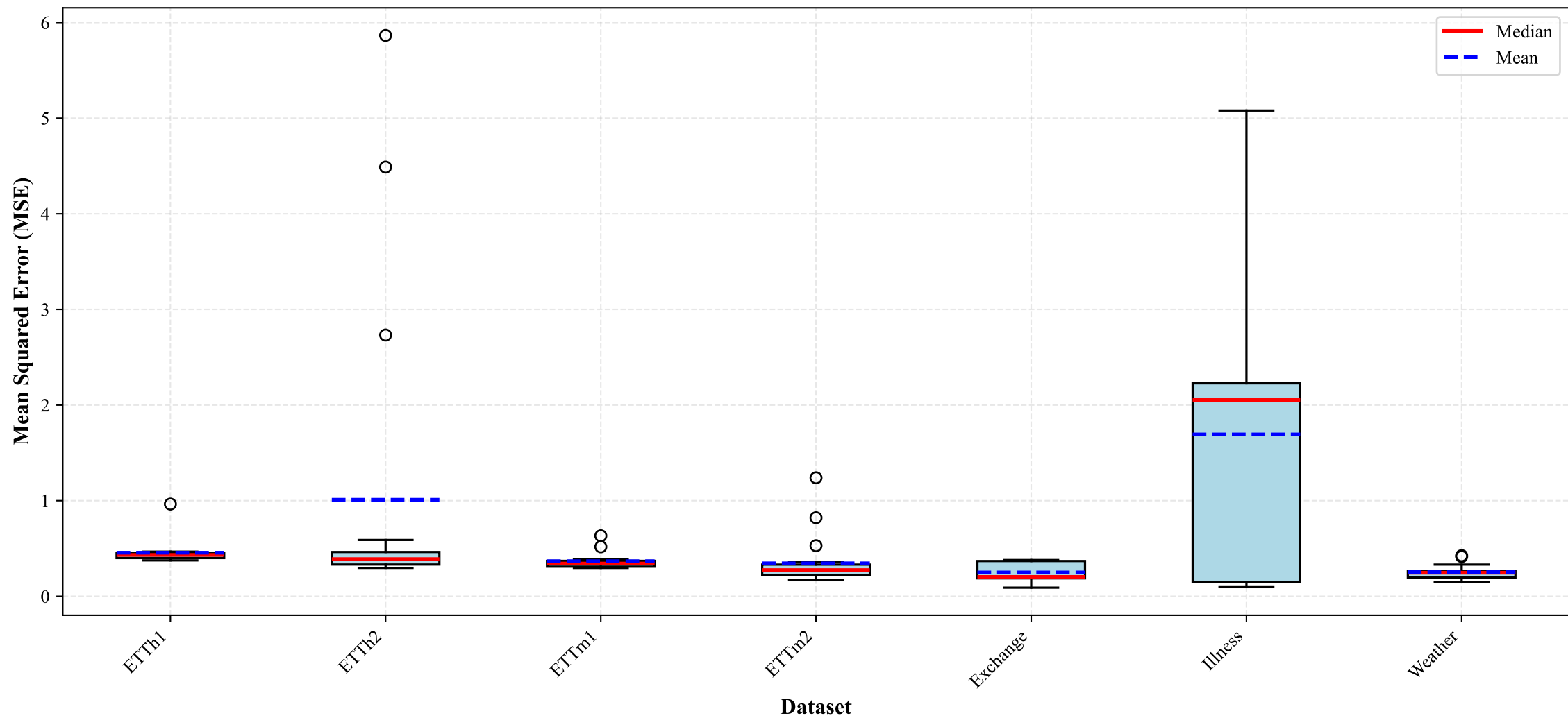
Performance Distribution Across Datasets (All Models)
