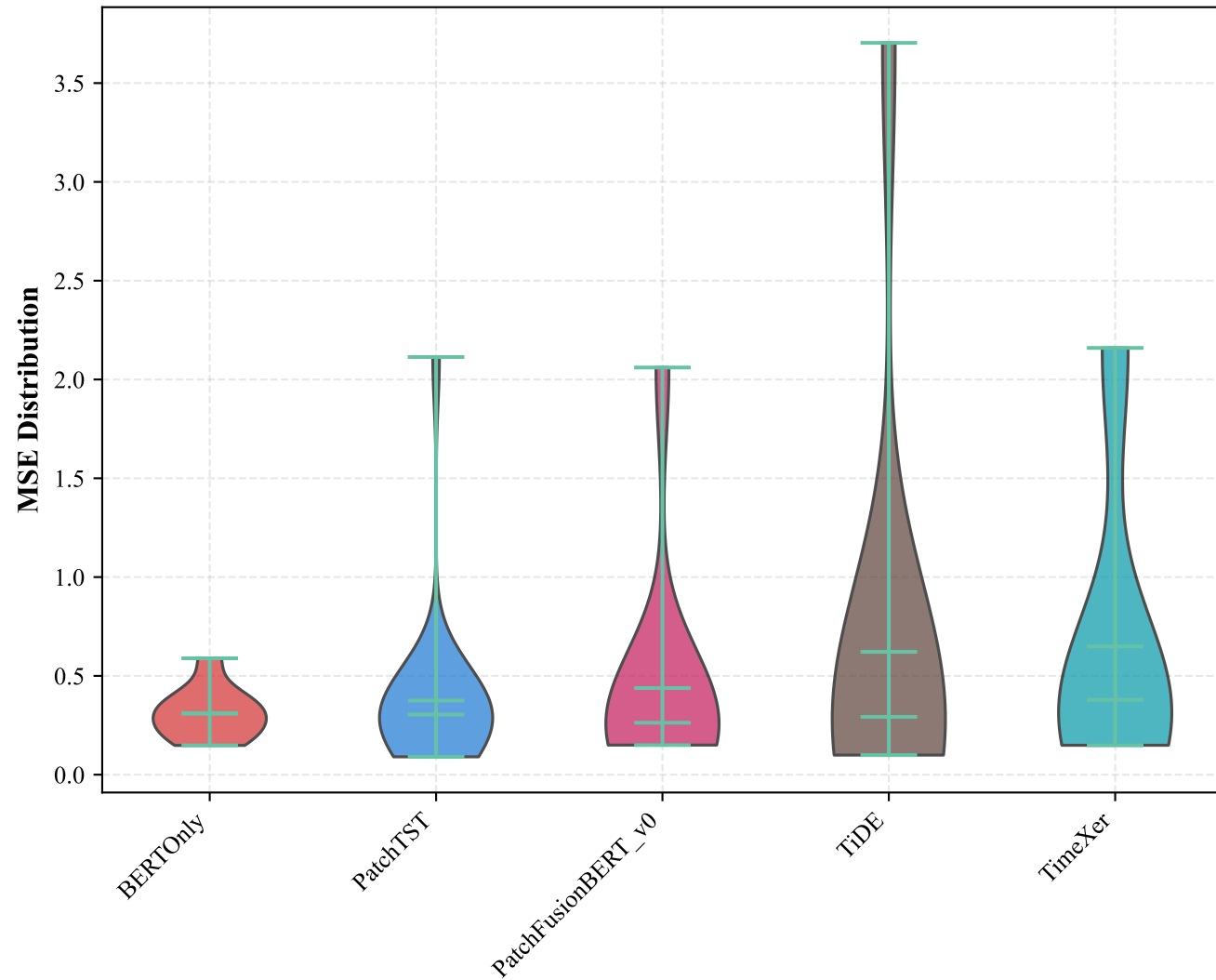
(a) MSE Distribution - Top 5 Models
