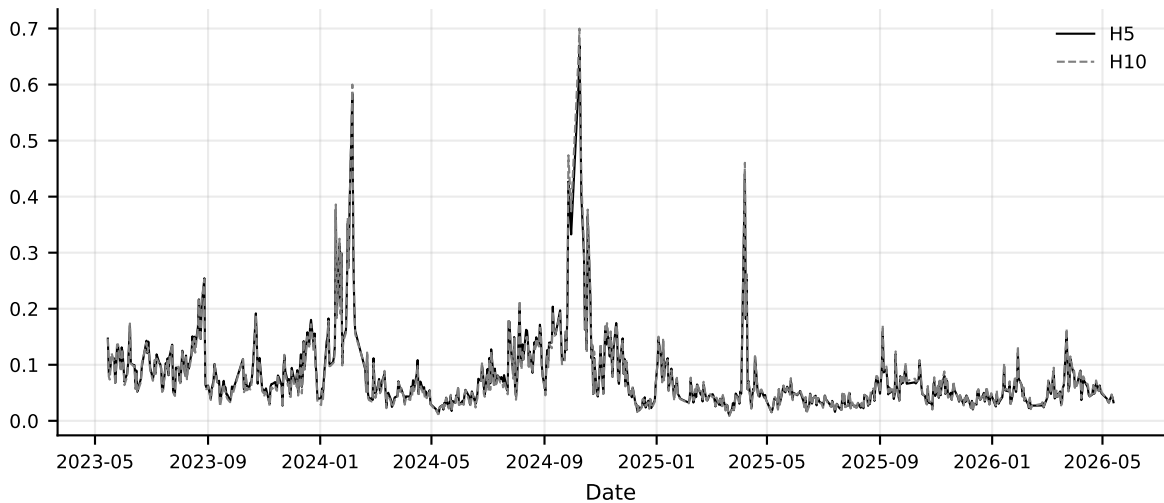
Daily onset event rate
