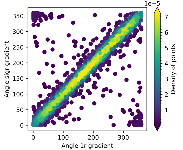
Figure 2: The comparison of the results from using the different methods for calculating the direction of velocity gradient.
