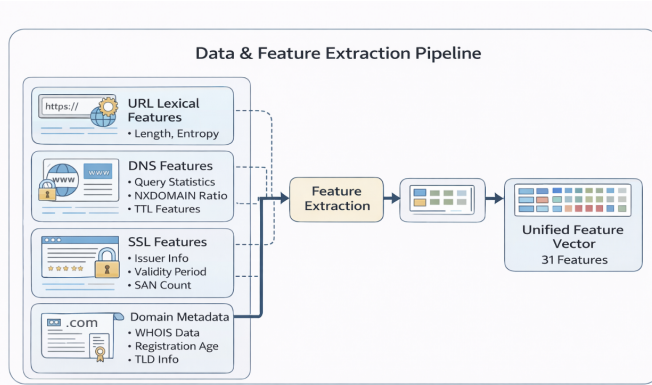
Fig. 2. Hybrid feature extraction pipeline combining multiple data sources.
