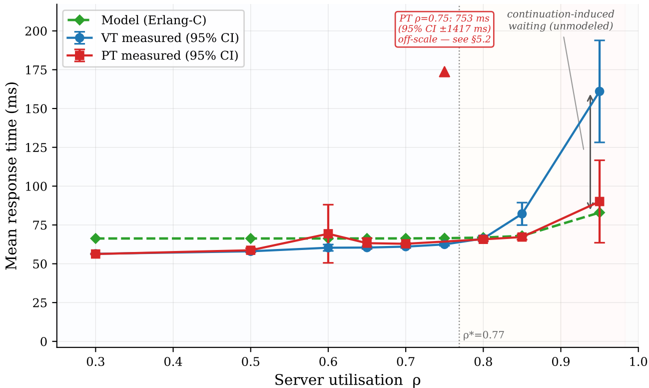
Mean Latency: Model Predictions vs Measurements (VT & PT)
