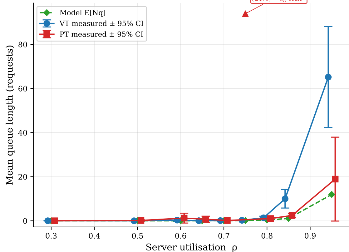
(b) Queue Length
