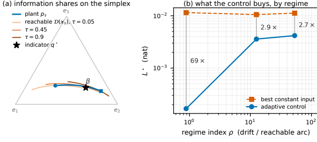
Figure 4: (a) The information-share curve p_\tau on the 2-simplex (circle: start, square: failure), the reachable sets D(x_\tau) at \tau = 0.05, 0.45 and 0.9 , and the optimal indicator q^* . No point lies on all three, so \beta cannot be held at zero (Theorem 4.1). (b) What steering buys, against the regime index \rho .
