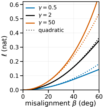
(a) exact vs. quadratic
