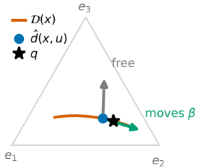
(b) cost of each motion
