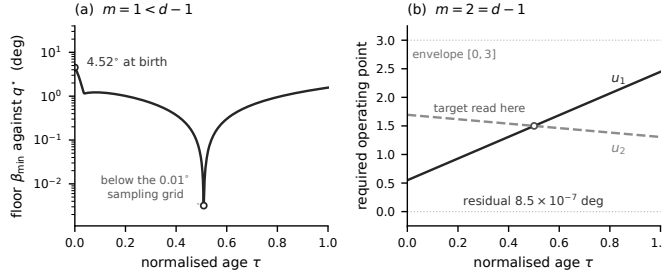
Figure 5: (a) With m = 1 the floor against q^* is largest at birth and dips below the sampling grid near mid-life. (b) With m = 2 the mid-life direction is held exactly; plotted is the operating point this requires, which never leaves \mathcal{U} .
