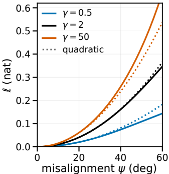
(a) exact and quadratic loss
