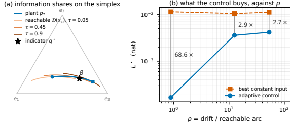
Figure 4: (a) The information-share curve p_\tau on the 2-simplex (circle: start, square: failure), the reachable sets \mathcal{D}(x_\tau) at \tau = 0.05, 0.45 and 0.9 , and the optimal indicator q^* . No point lies on all three, so \beta cannot be held at zero (Theorem 4.1). (b) What steering buys, against \rho , the drift of the reachable arc over its length.
