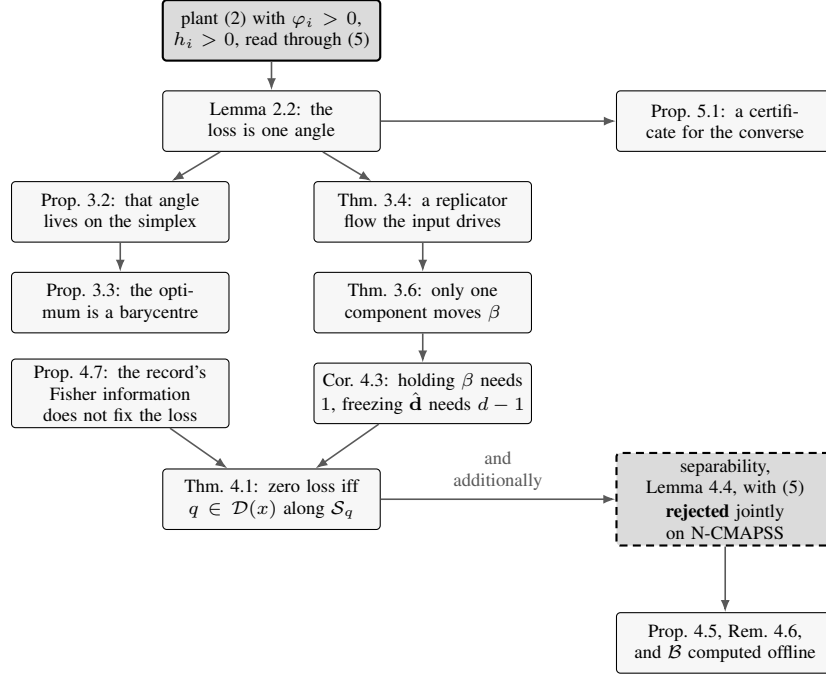
Figure 6: What rests on what. The spine needs only the positivity of \mathbf{d} , which the degradation model gives in the channel coordinates of (5). The dashed branch adds separability. Section 7 reports the two rejected jointly on raw turbofan sensors, which keeps those sensors off the spine as well until the observation map is inverted.
