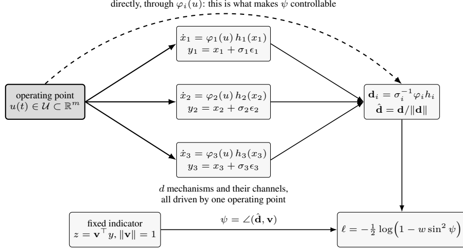
Alignment asks \hat{d}(x, u) = q : d - 1 scalar equations on m unknowns, whence the counting rule of Theorem 4.1.
