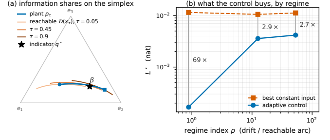
Figure 4: (a) The information-share curve p_\tau on the 2-simplex (circle: start, square: failure), the reachable sets \mathcal{D}(x_i) at \tau = 0.05, 0.45 and 0.9 , and the optimal indicator q^* . No point lies on all three, so \beta cannot be held at zero (Theorem 4.1). (b) What steering buys, against the regime index \rho .
