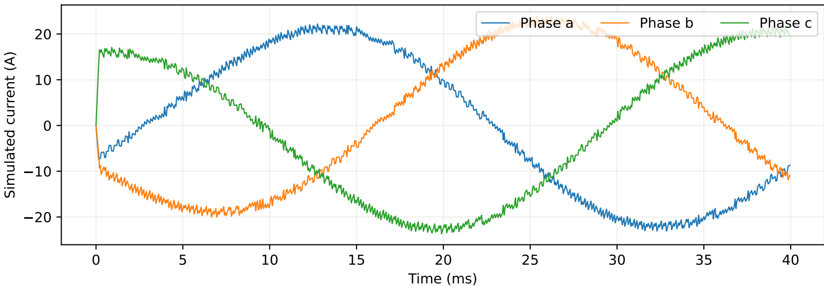
Independent ngspice T-type circuit: healthy 25 °C
