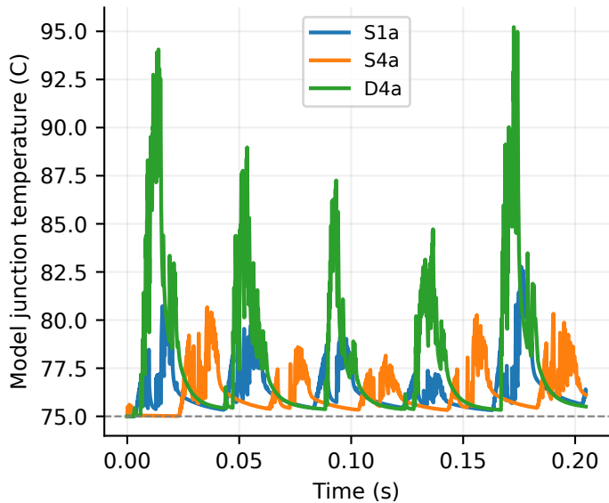
Fixed 75 C case, conduction heat
