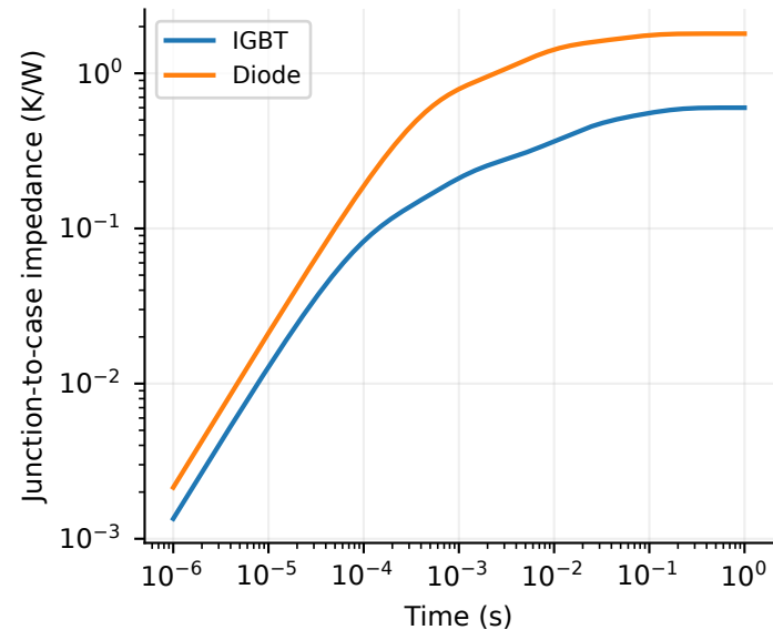
Datasheet Foster coefficients
