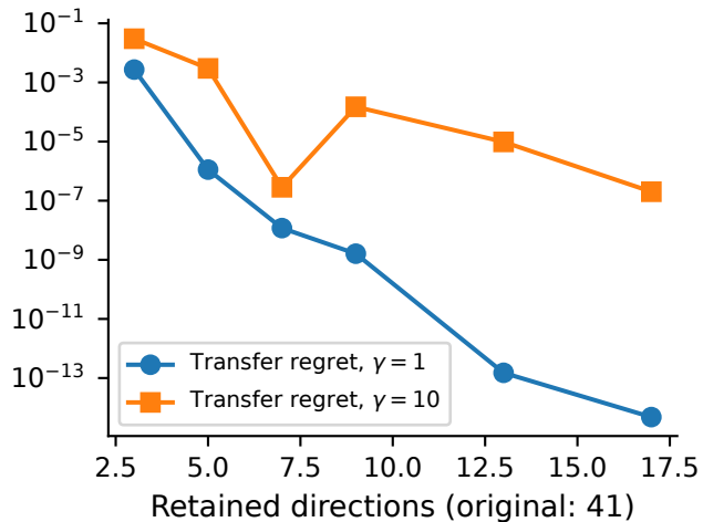
Achieved regret (nats)
