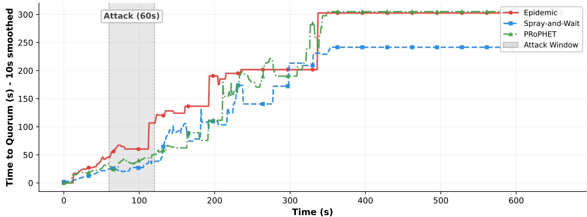
Comparison of Routing Protocols under RF Jamming Attack (loss=80%) - Latency
