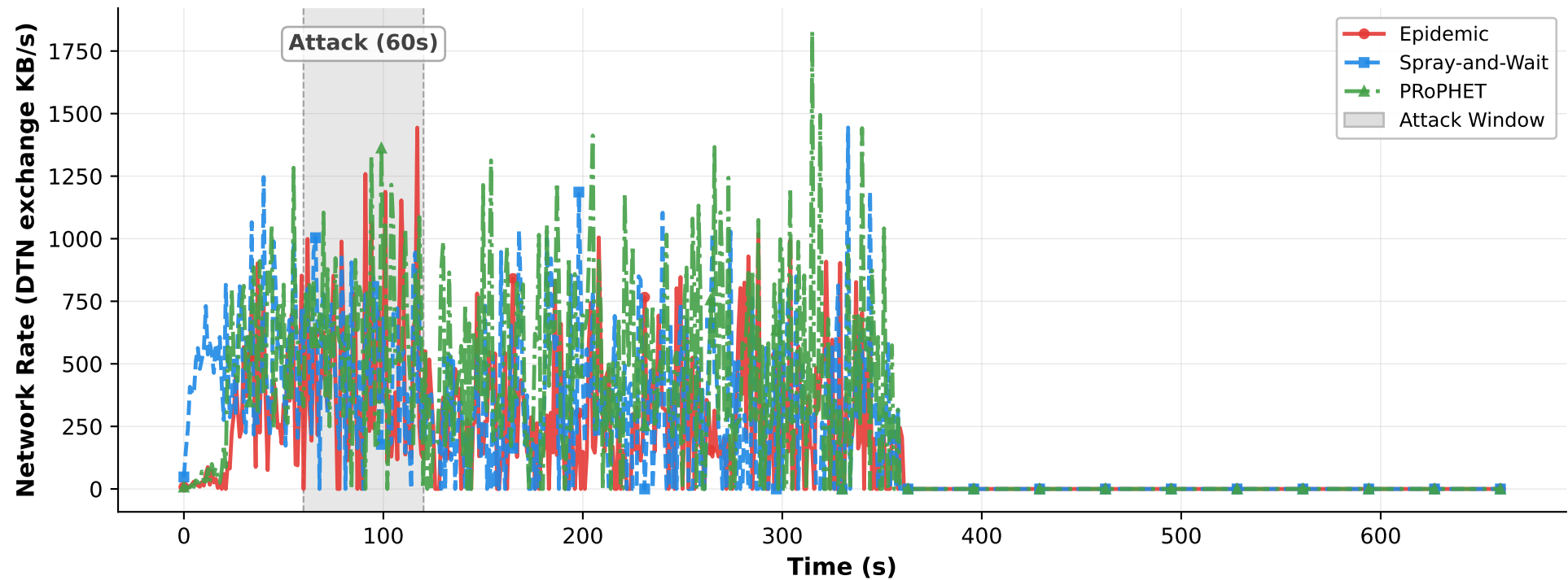
Comparison of Routing Protocols under RF Jamming Attack (loss=80%) - Throughput
