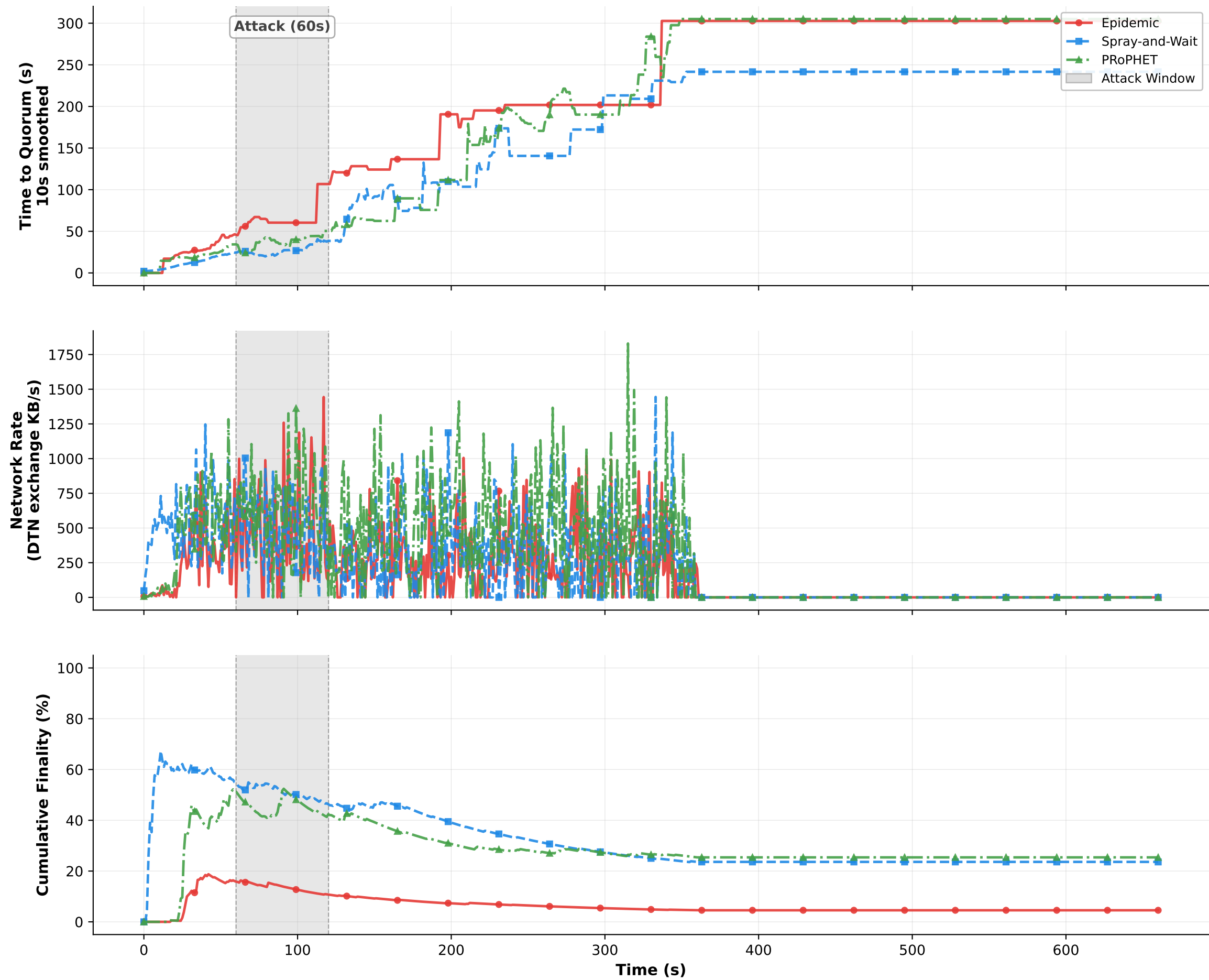
Comparison of Routing Protocols under RF Jamming Attack (loss=80%)
