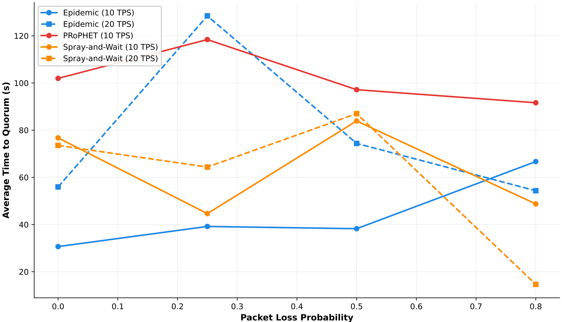
Average Quorum Latency vs. Packet Loss under Attack
