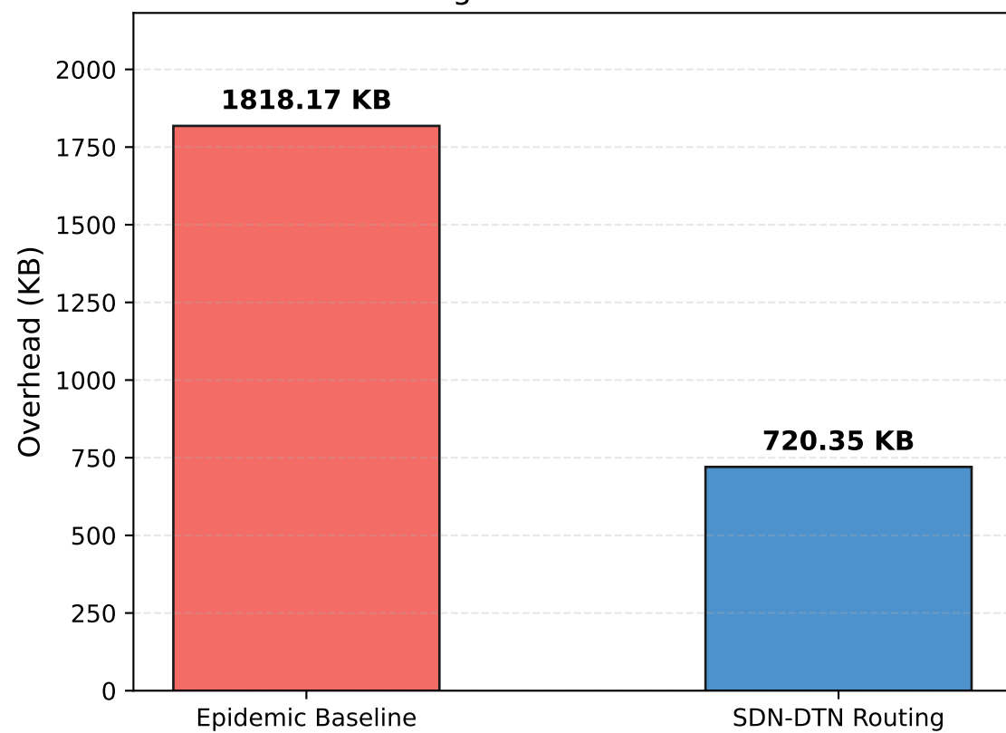
Routing & Control Overhead
